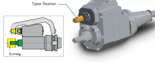
Angular Head
