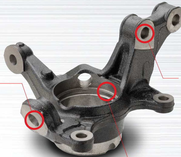
02 Finishing of Bearing Hole
